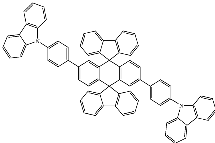
Chemical Compound 403
