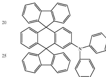
Chemical Compound 7
