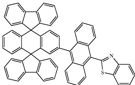
Chemical Compound 214
