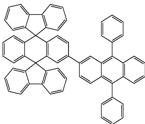
Chemical Compound 116
