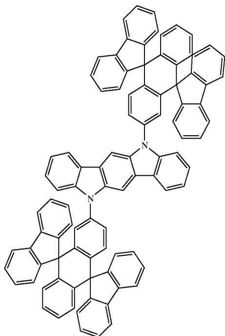
Chemical Compound 405
