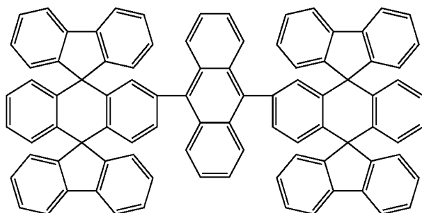
Chemical Compound 103
