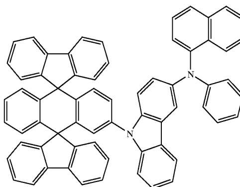
Chemical Compound 306
