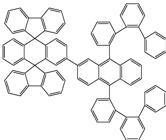
Chemical Compound 137
