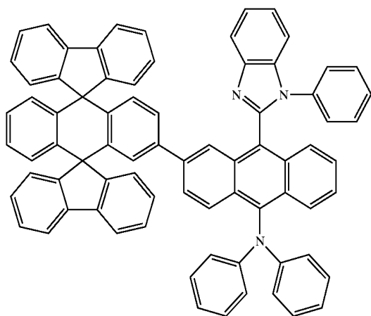
Chemical Compound 127
