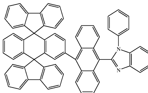
Chemical Compound 202
