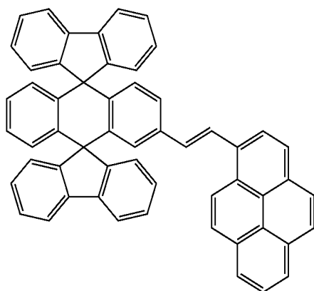
Chemical Compound 105
