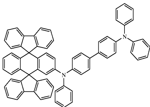
Chemical Compound 400
