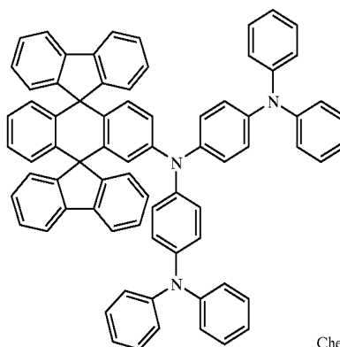
Chemical Compound 400
