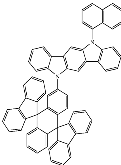
Chemical Compound 413
