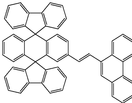
Chemical Compound 104
