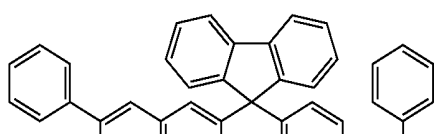
Chemical Compound 105
