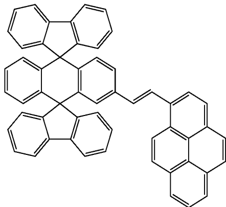
Chemical Compound 103
