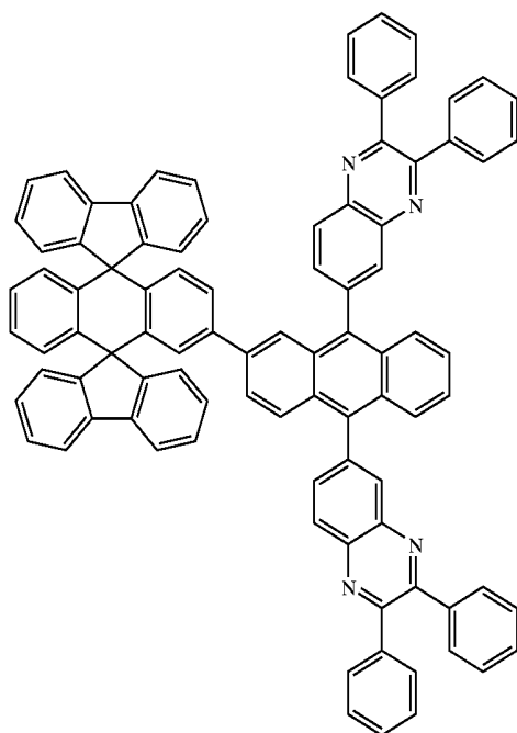
Chemical Compound 212
