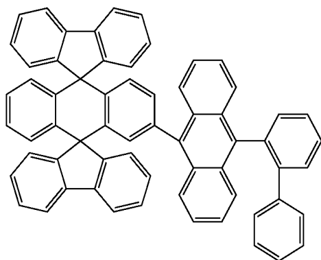
Chemical Compound 111
