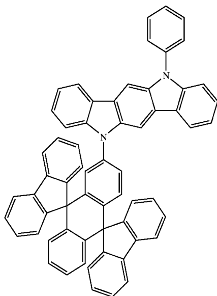
Chemical Compound 412
