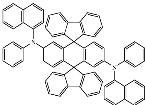
Chemical Compound 302
