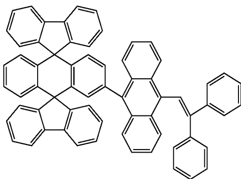
Chemical Compound 201
