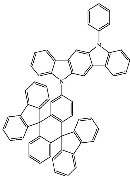
Chemical Compound 410
