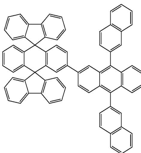
Chemical Compound 119
