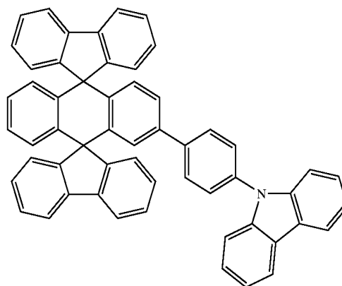
Chemical Compound 406
