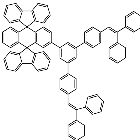
Chemical Compound 108
