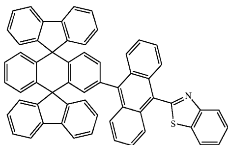
Chemical Compound 214
