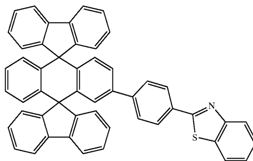
Chemical Compound 213
