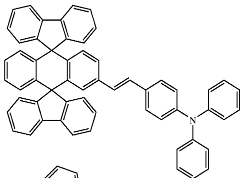
Chemical Compound 400
