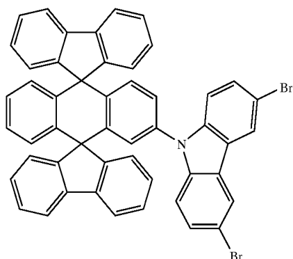
Chemical Compound 7
