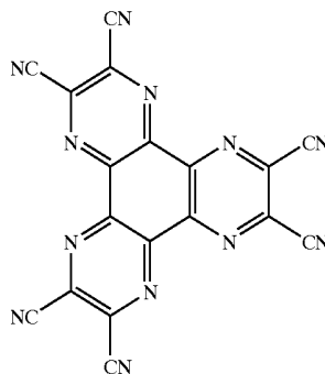
Hexanitrile hexaazatriphenylene
