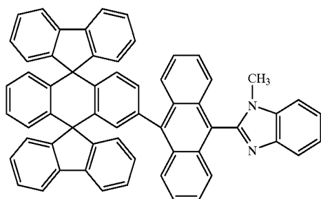
Chemical Compound 205
