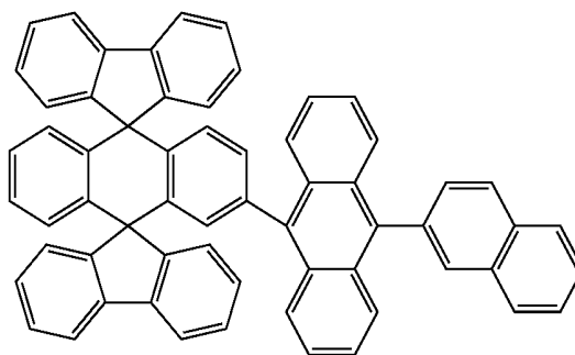
Chemical Compound 112
