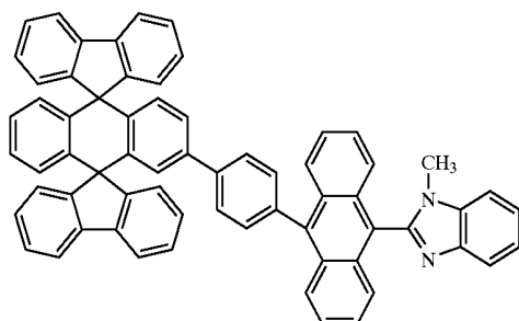
Chemical Compound 201
