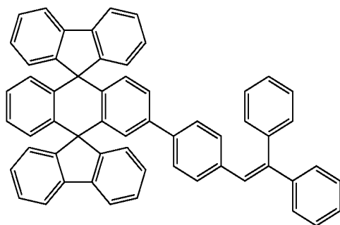
Chemical Compound 107
