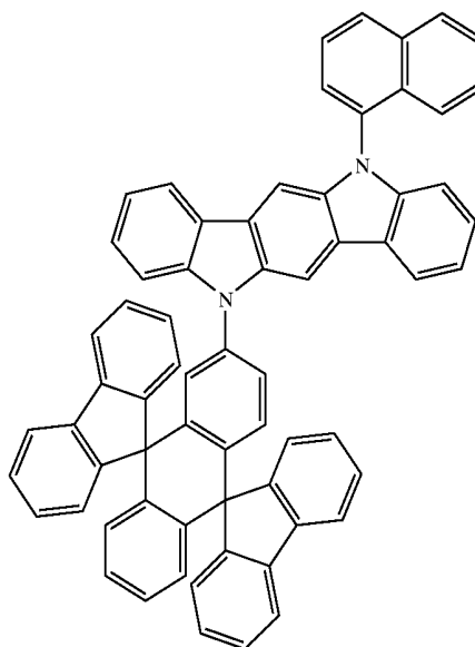
Chemical Compound 411
