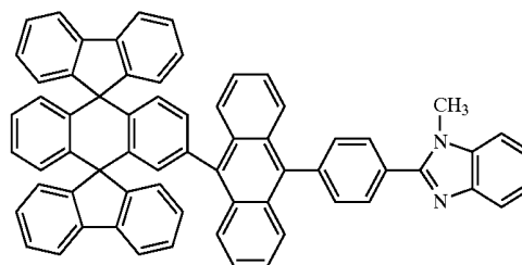
Chemical Compound 209
