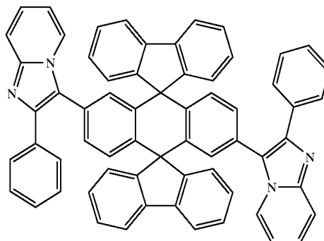
Chemical Compound 413
