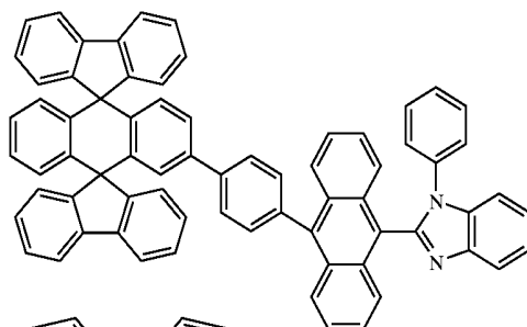
Chemical Compound 207
