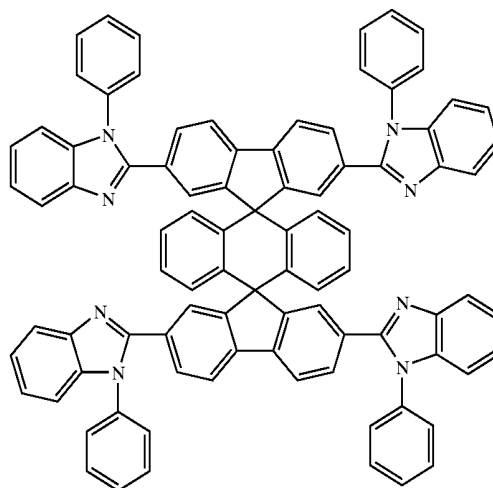
Chemical Compound 219
