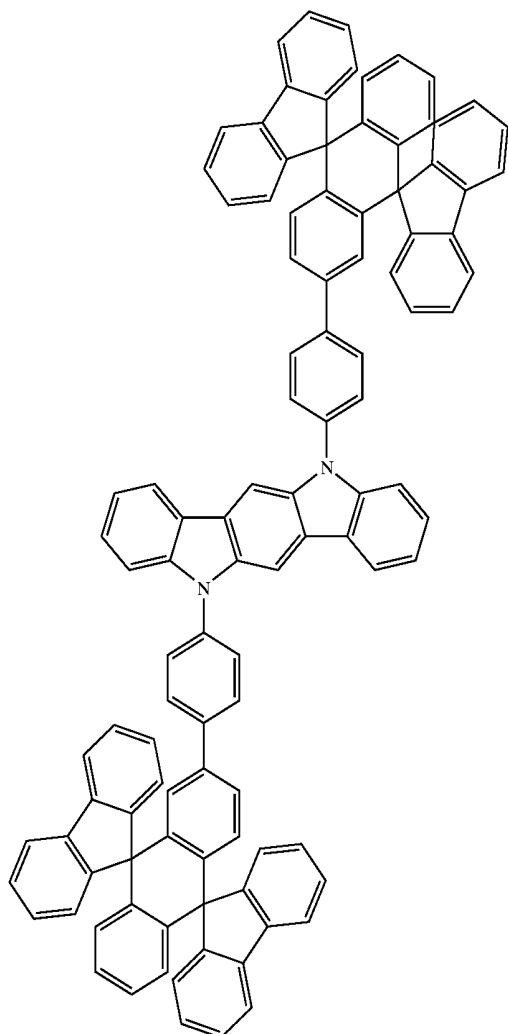
Chemical Compound 410
