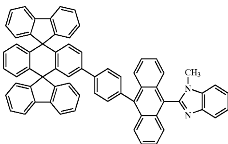
Chemical Compound 201
