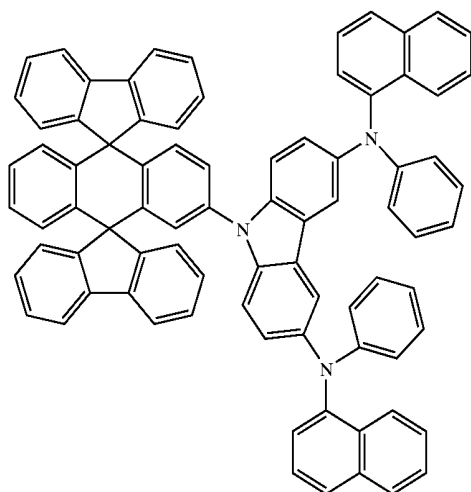
Chemical Compound 405
