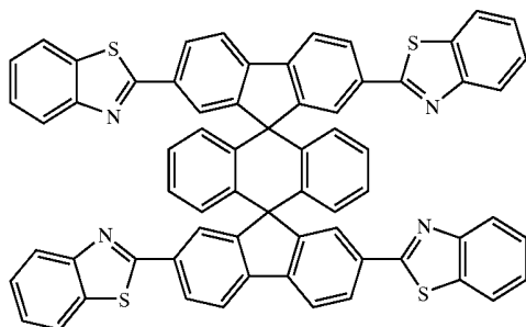
Chemical Compound 218
