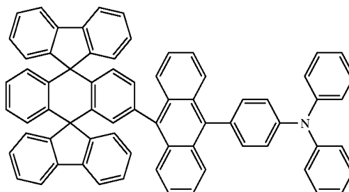
Chemical Compound 402
