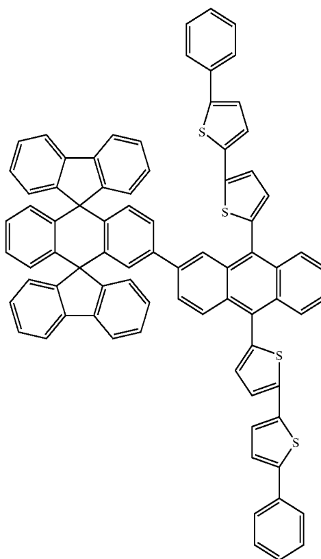
Chemical Compound 128
