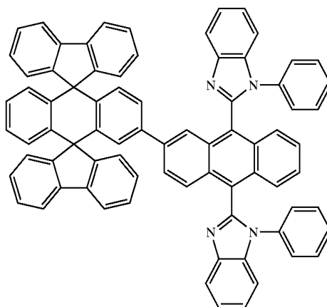
Chemical Compound 202
