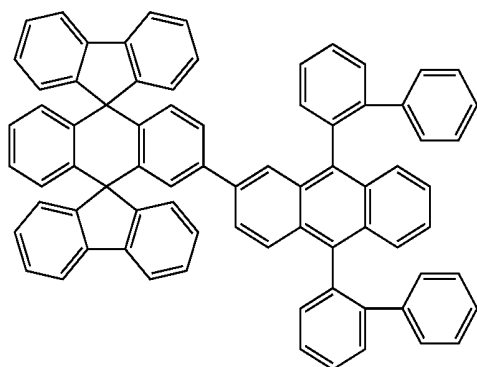
Chemical Compound 118
