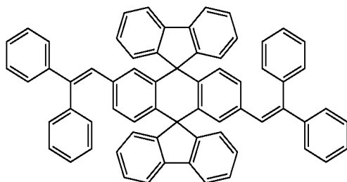
Chemical Compound 105
