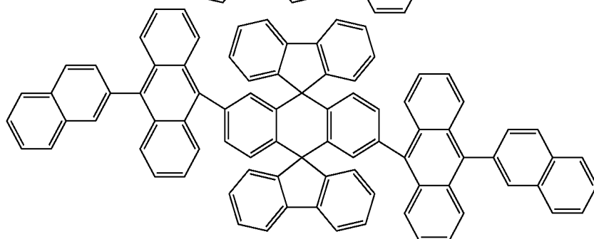
Chemical Compound 116
