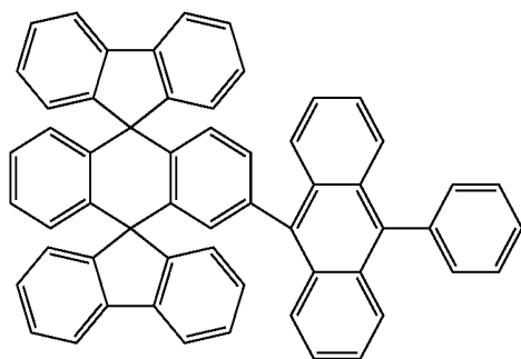
Chemical Compound 111
