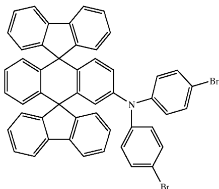
Chemical Compound 8
