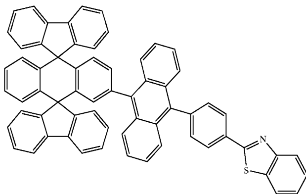
Chemical Compound 218
