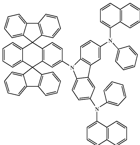
Chemical Compound 403
